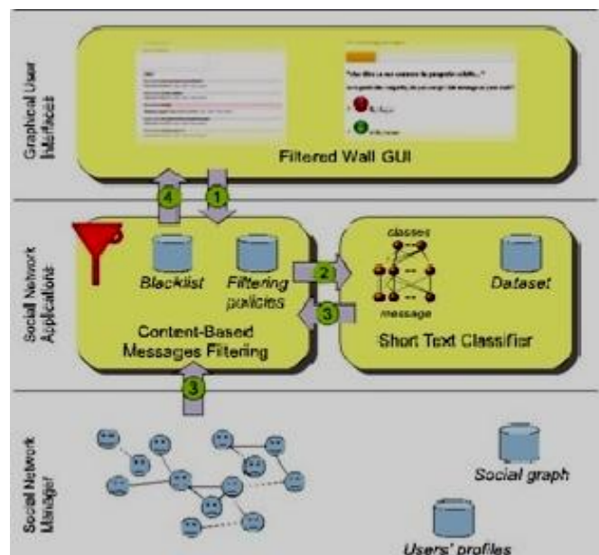
Fig.1: General Architecture of online Social Network
