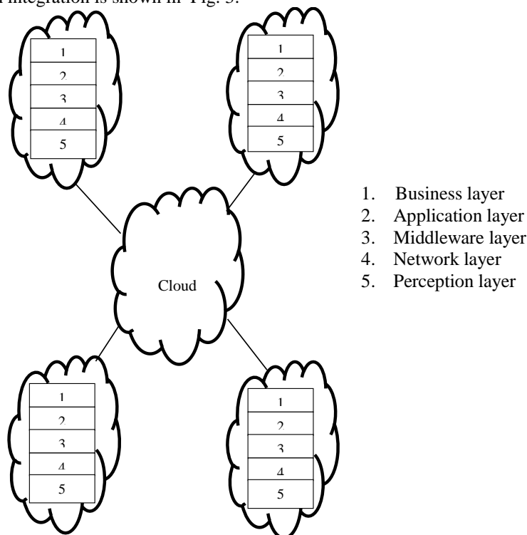
Fig.3 Data communication between Cloud and IoT
