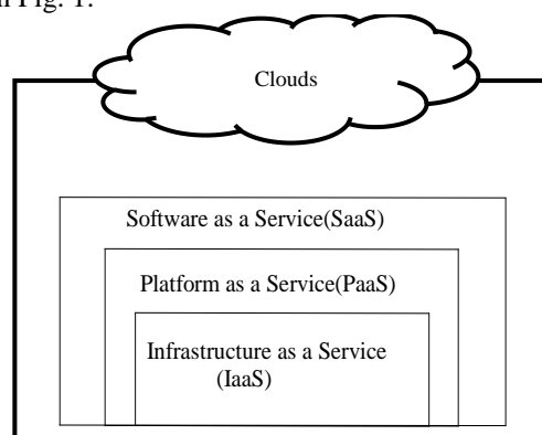
Fig. 1 Services Stack
