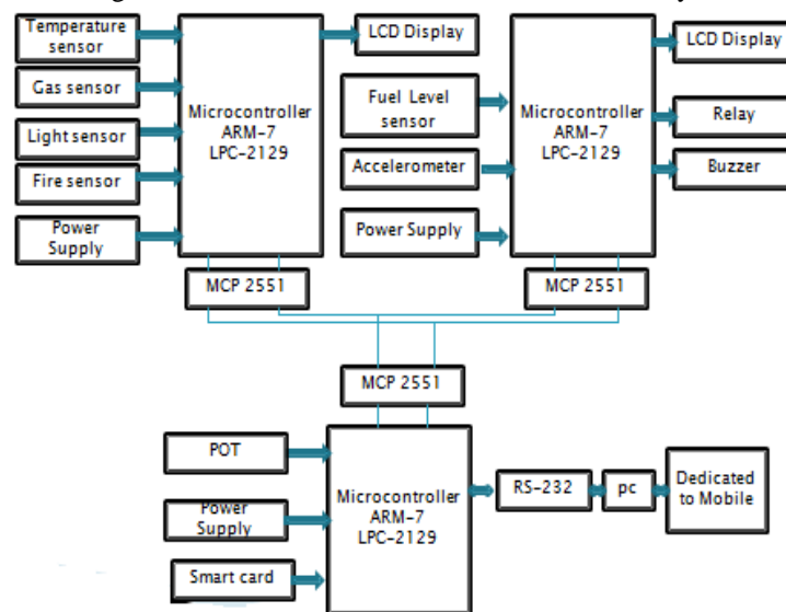
Figure 2: Block diagram of CAN based industrial parameter monitoring system.
