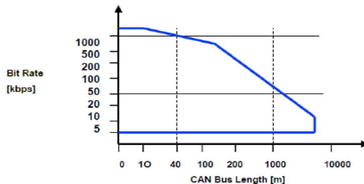
Figure 3: CAN bus length versus bit rate
