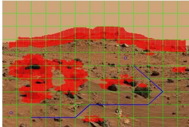
Fig.6. Path Planning
