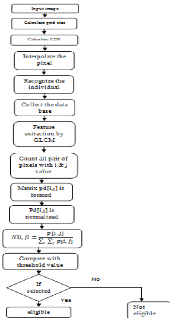
Fig 4.1: This flow chart describes the entire process involved in AHE technique, GLCM algorithm and neural network
