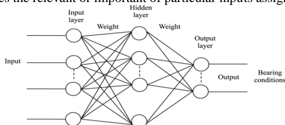
Fig 1.1: neural network architecture
