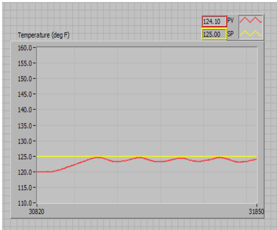
Figure 7. Minimal offset with oscillation.
