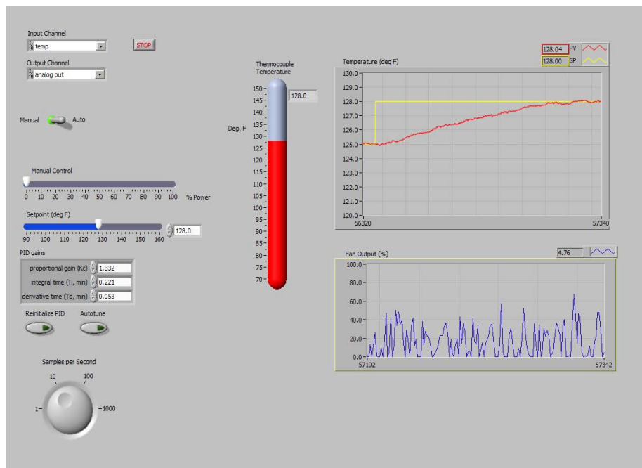
Figure 8. Autotuned PID Loop Response to Set point Step Change.
