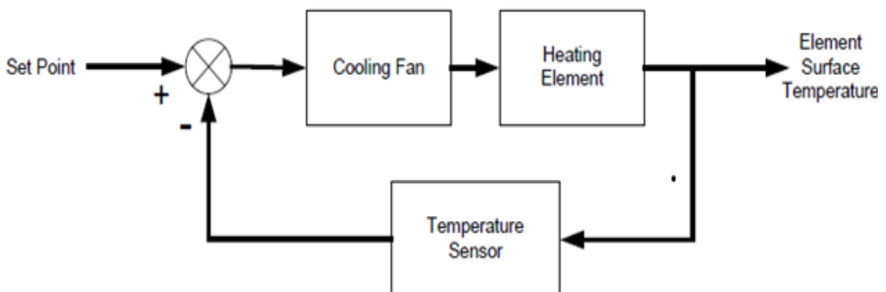
Figure 1. Feedback System Block Diagram
