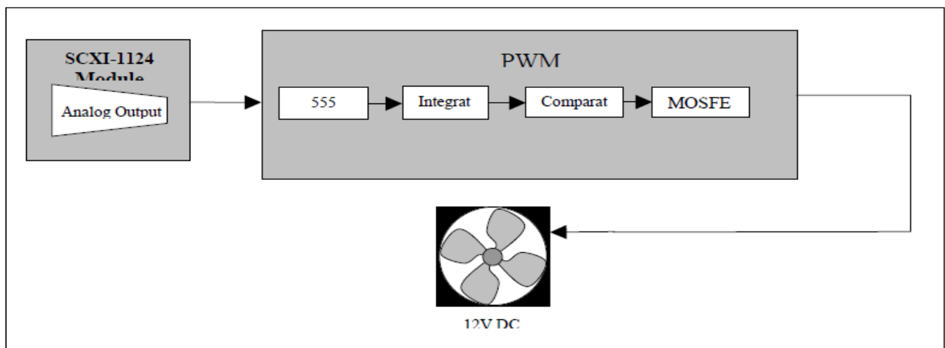
Figure 4. DC Fan Connected To Interface Circuit
