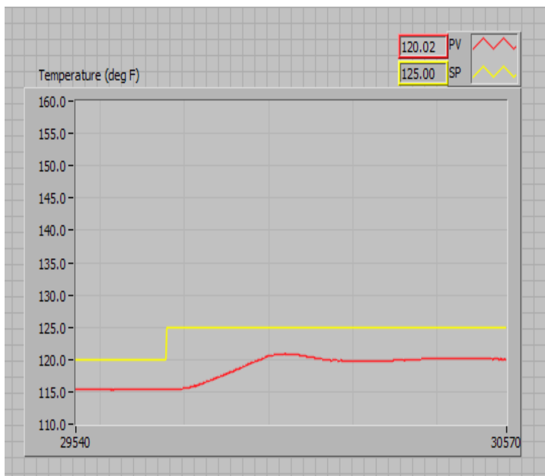
Figure 6. Proportional-only control, unity gain.
